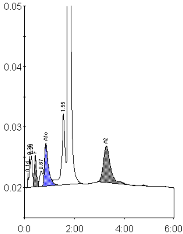
Peak table - ID: 10364892
